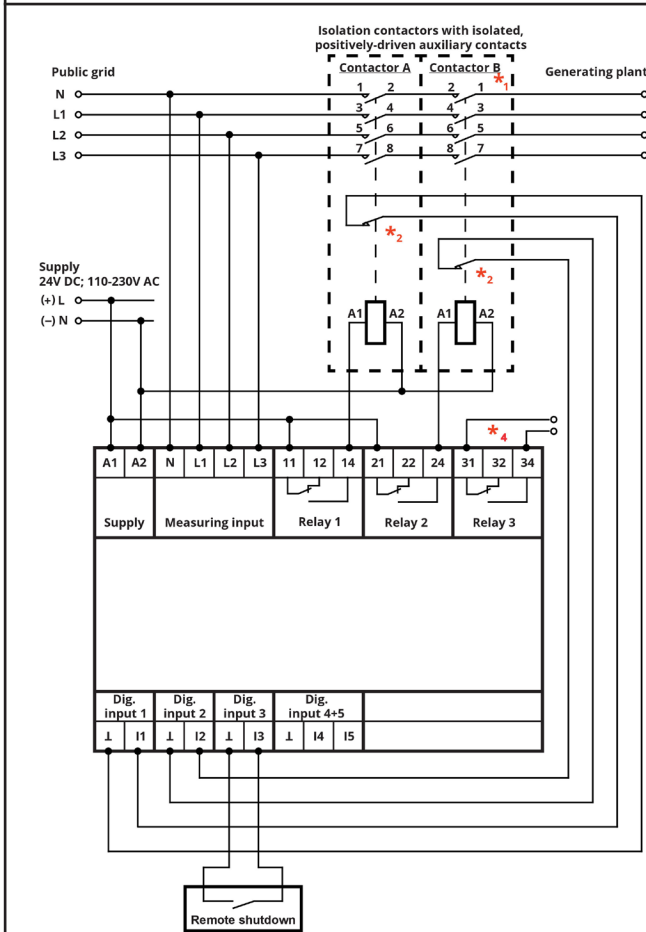
Connection diagram 1:
