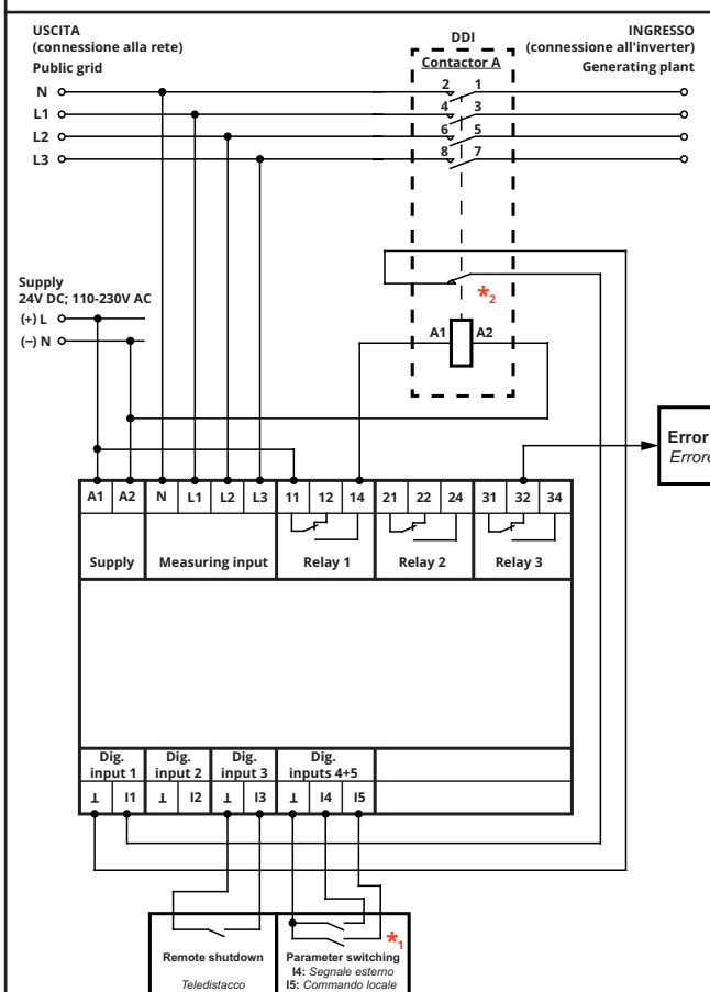
Connection diagram 2:
