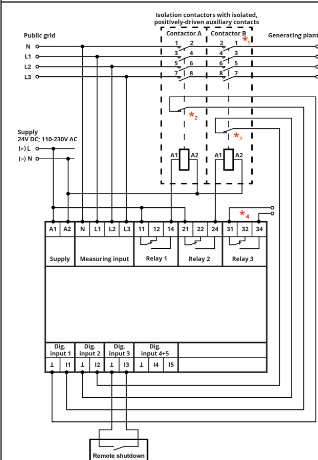
Connection diagram 1:
