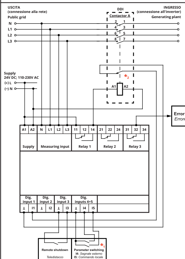
Connection diagram 2:
